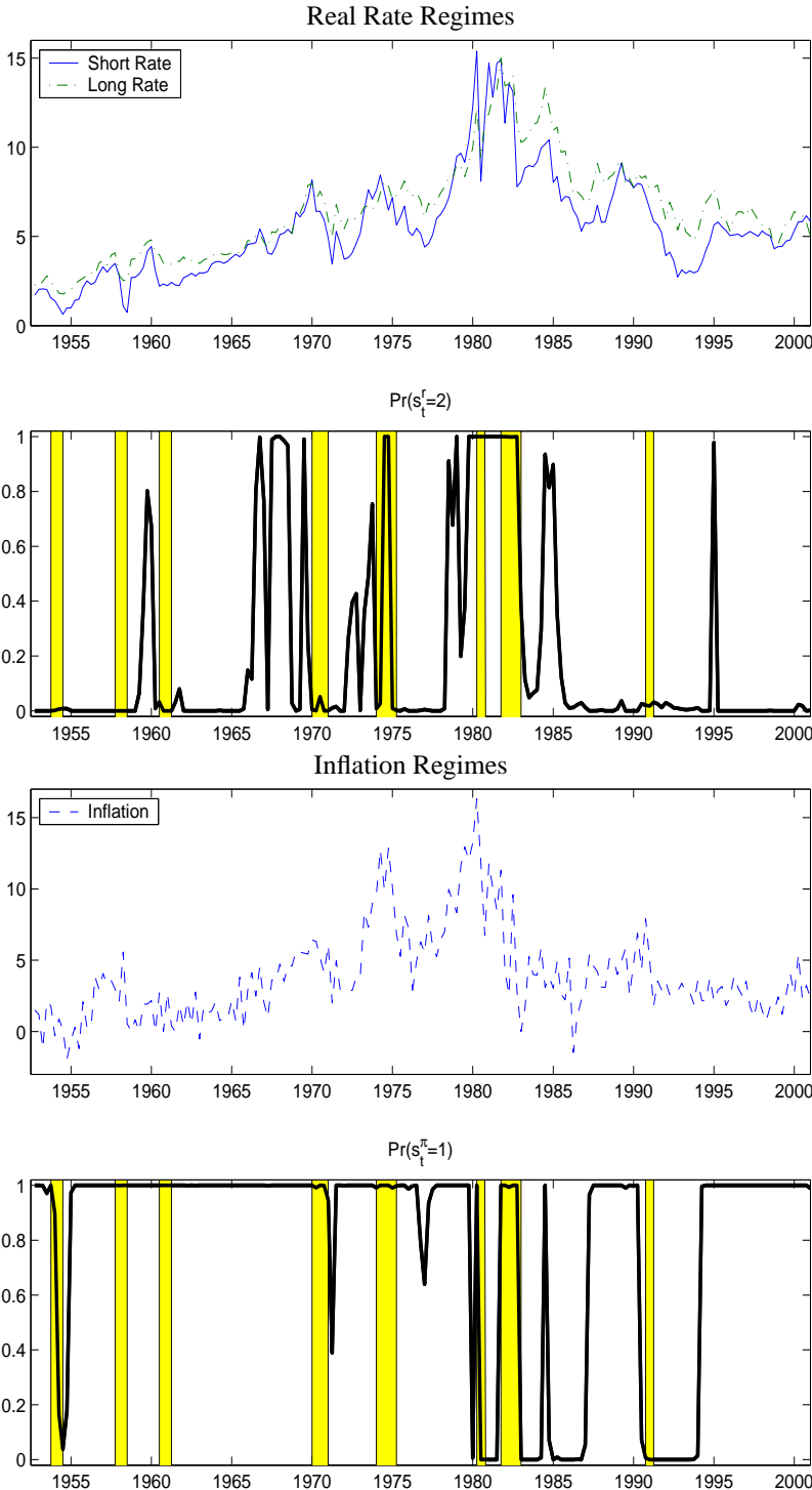
Figure 3: Smoothed Regime Probabilities: Independent Real Rate and Inflation Regimes
